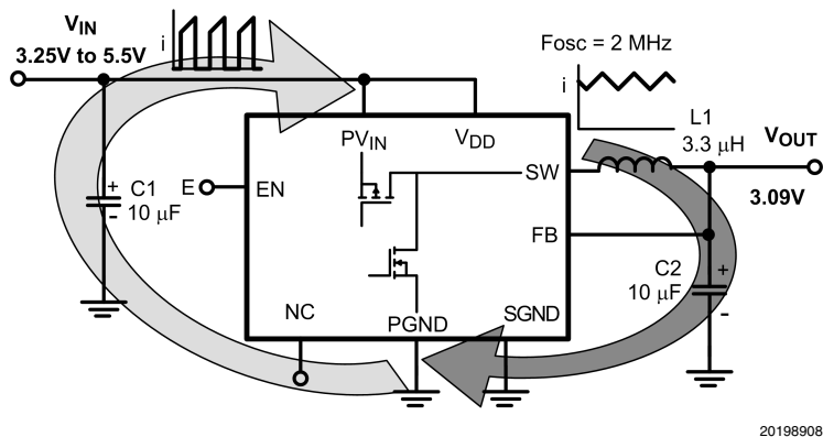
FIGURE 4. Current Loop
