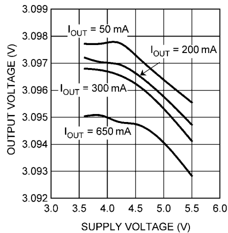
Output Voltage vs Supply Voltage ( V_{OUT} = 3.09V )
